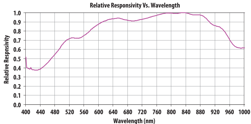
Figure 22. Wavelength Responsivity
